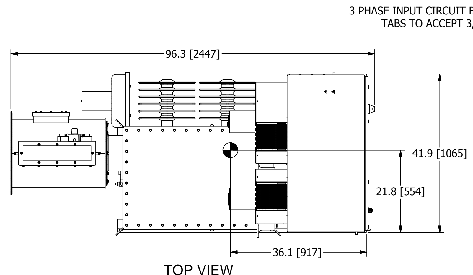
TOP VIEW
