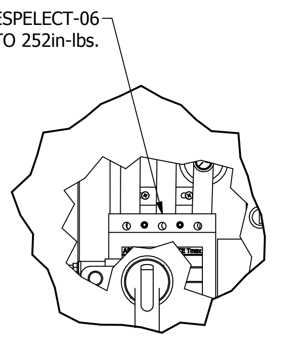
DETAIL C CIRCUIT BREAKER DETAIL SCALE 1 / 5
