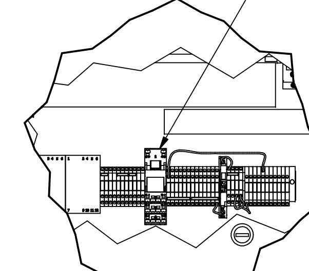
DETAIL D '2TB' TERMINAL BLOCK RAIL ASSEMBLY SCALE 1/5
