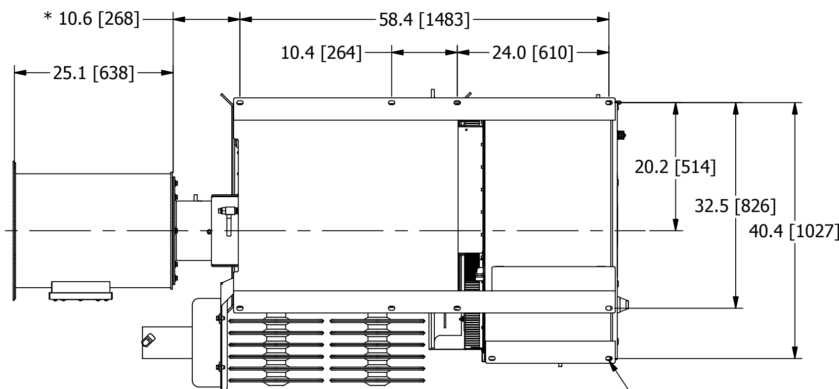
MOUNTING ARRANGEMENT FROM BOTTOM VIEW (VIEW B-B)
