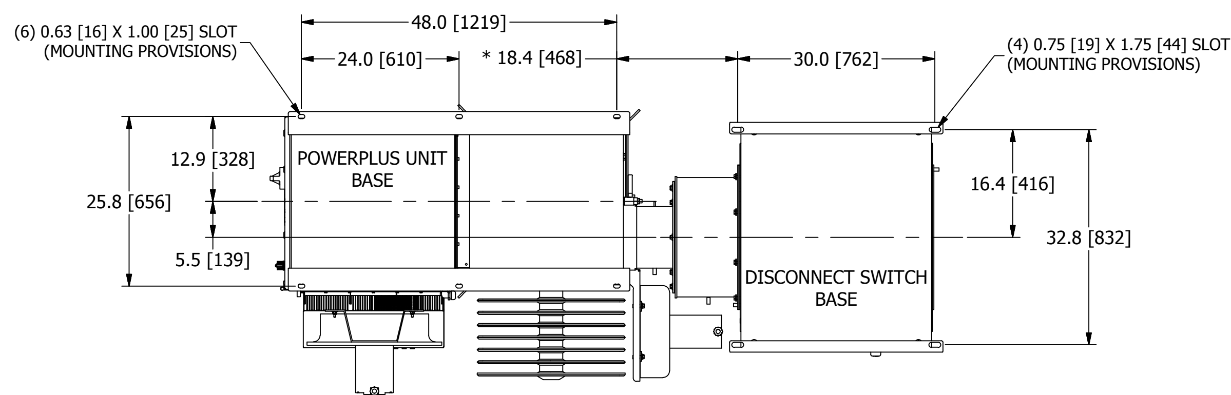
MOUNTING ARRANGEMENT FROM BOTTOM VIEW (SECTION B-B)
