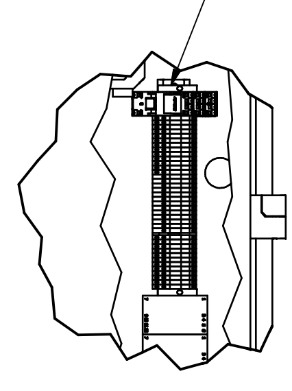
DETAIL D '2TB' TERMINAL BLOCK RAIL ASSY SCALE 1 / 6
