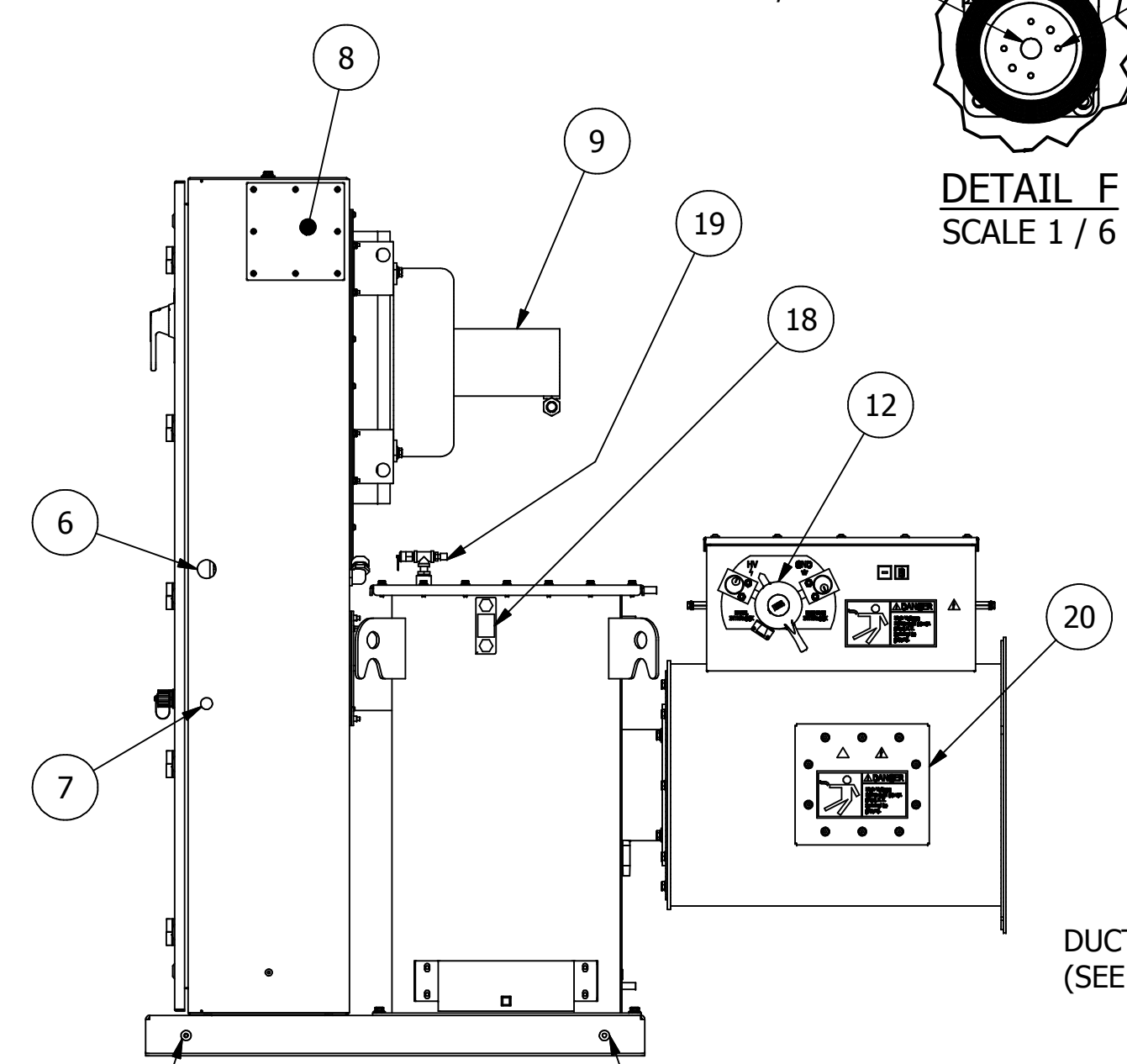
RIGHT VIEW
