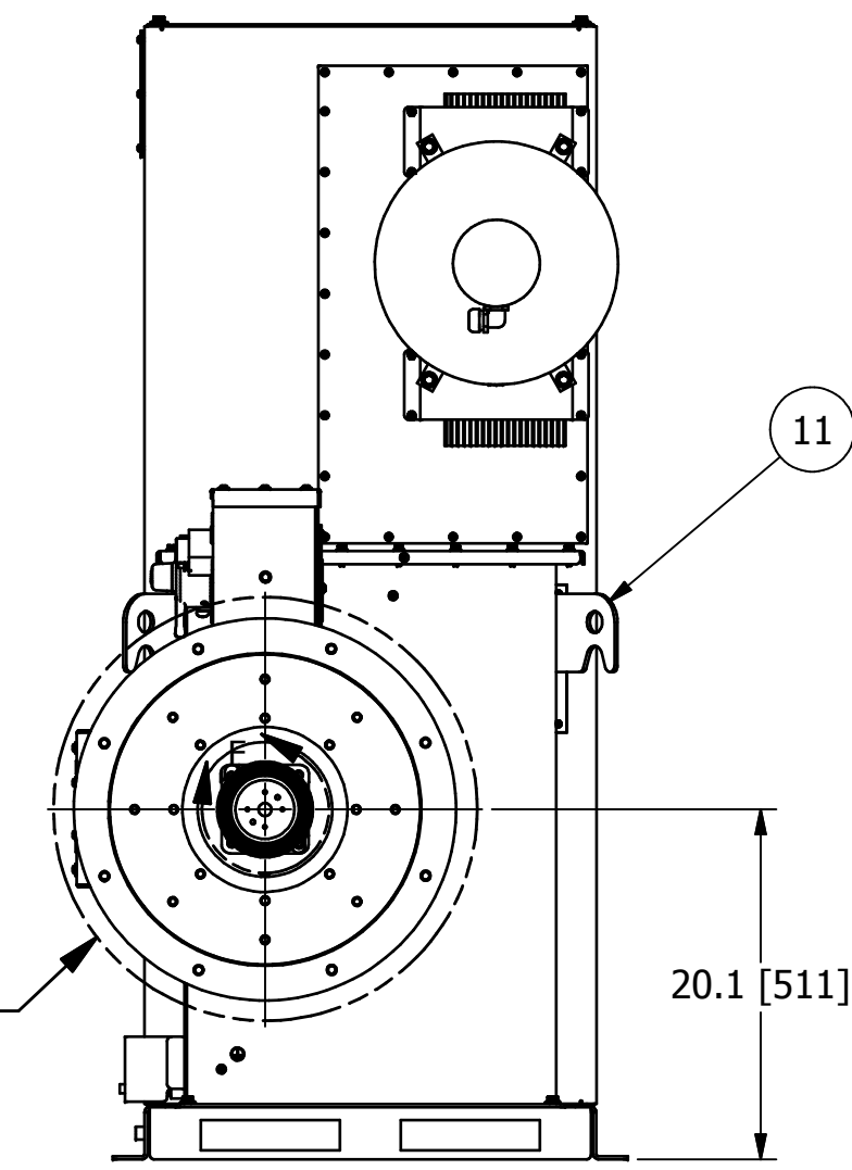
REAR VIEW
