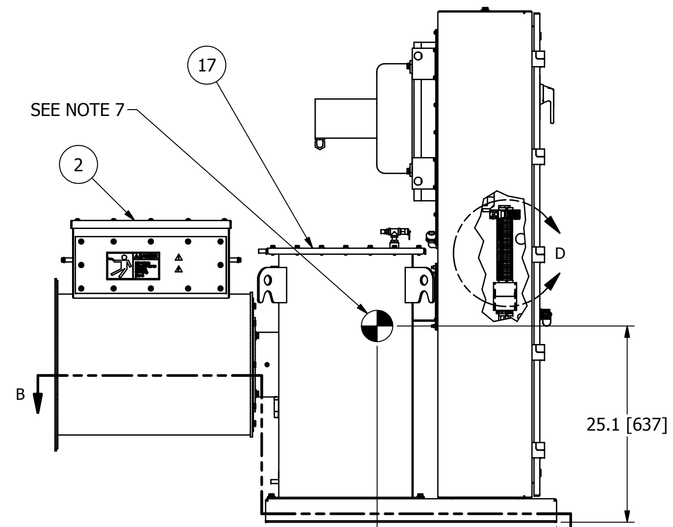
LEFT VIEW
