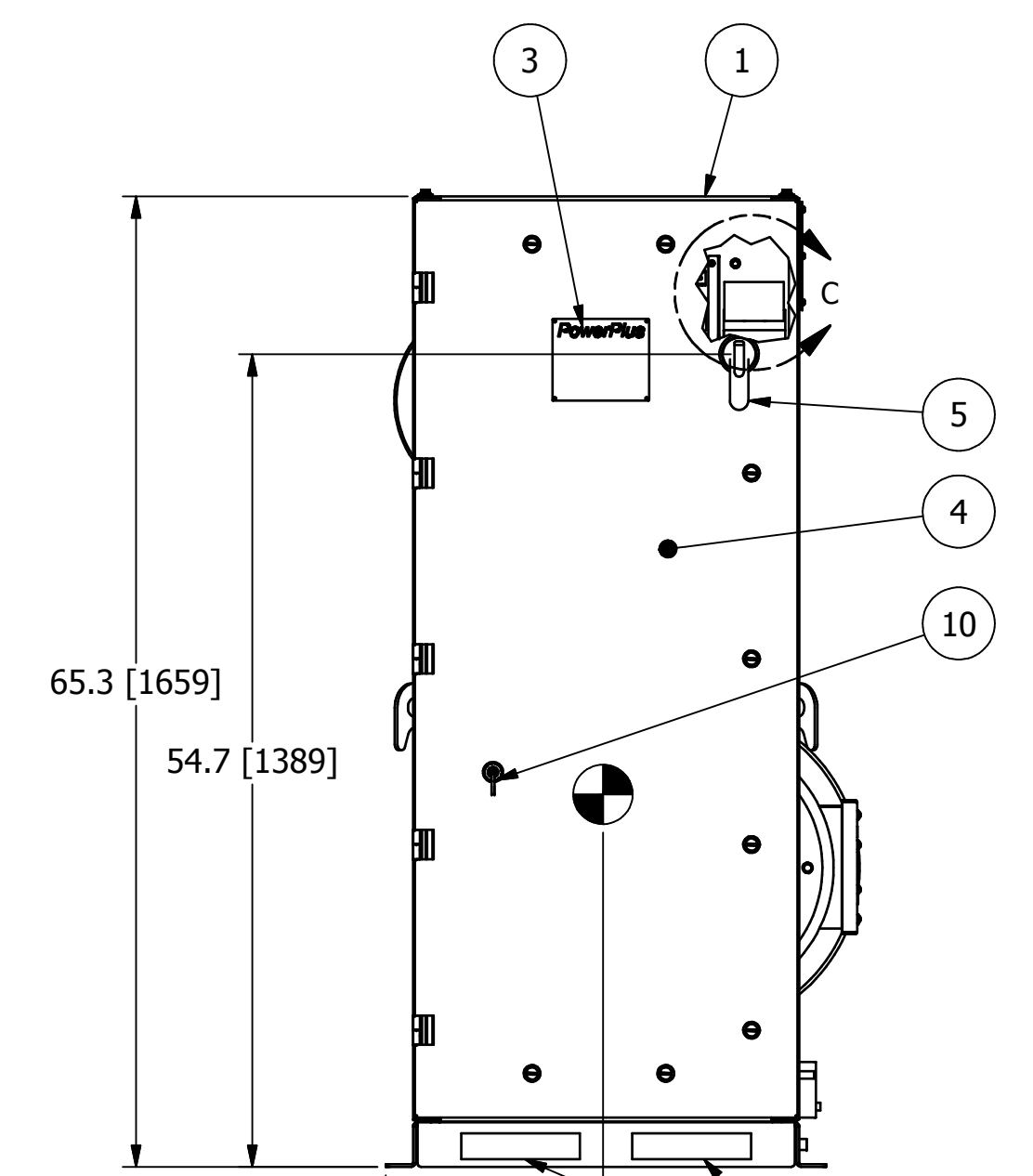
FRONT VIEW
