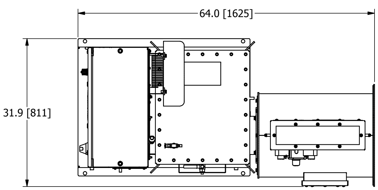
TOP VIEW
