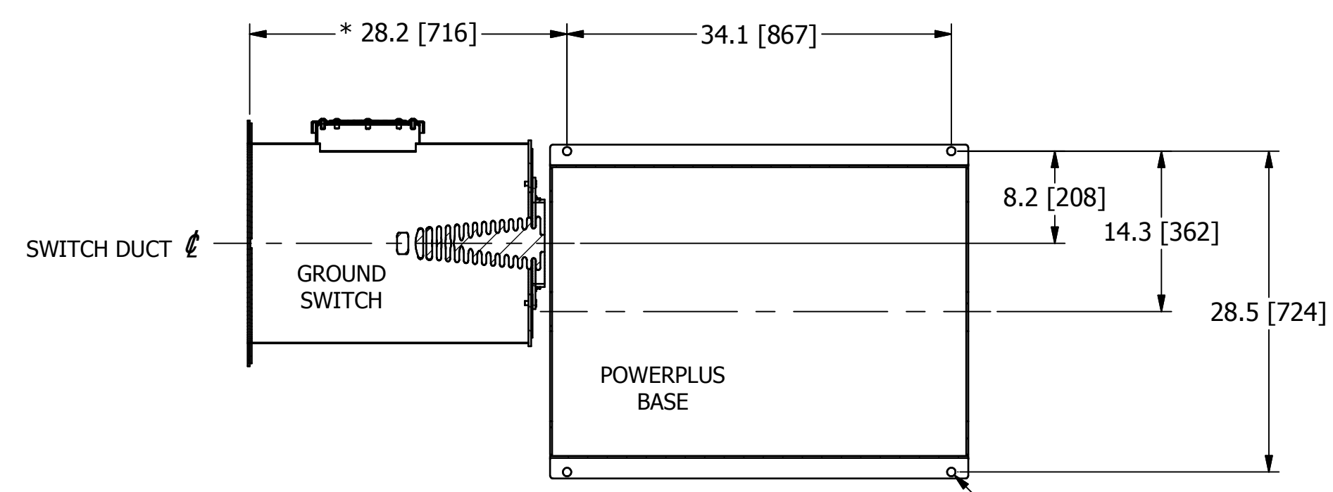
MOUNTING ARRANGEMENT FROM TOP VIEW (SECTION B-B)
