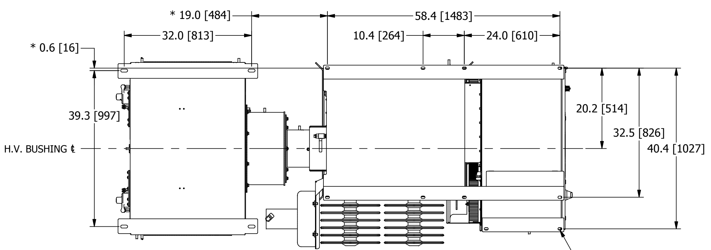
MOUNTING ARRANGEMENT FROM BOTTOM VIEW (VIEW B-B)
