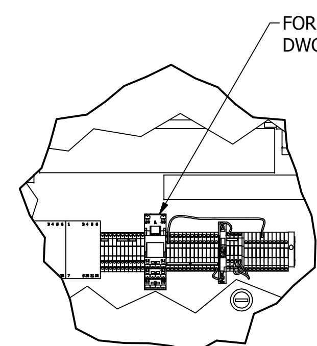
DETAIL D '2TB' TERMINAL BLOCK RAIL ASSEMBLY SCALE 1 / 5
