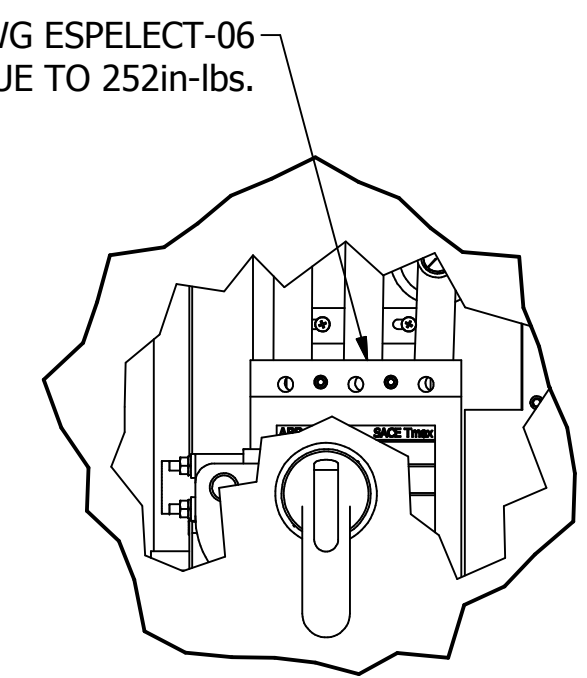
DETAIL C CIRCUIT BREAKER DETAIL SCALE 1 / 5
