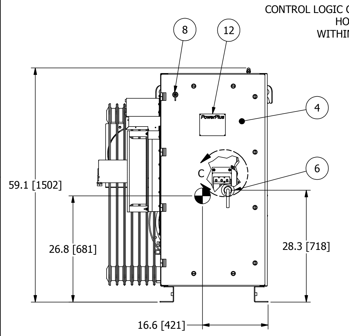
FRONT VIEW
