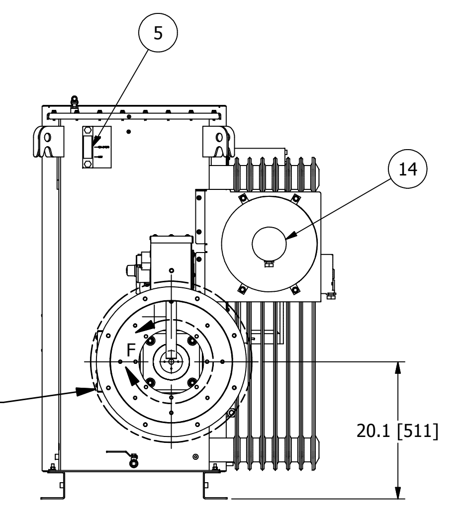
REAR VIEW
