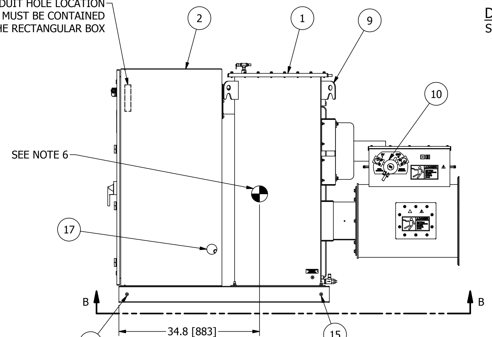
RIGHT VIEW
