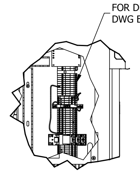
DETAIL D TERMINAL BLOCK RAIL ASSEMBLY SCALE 1 / 6
