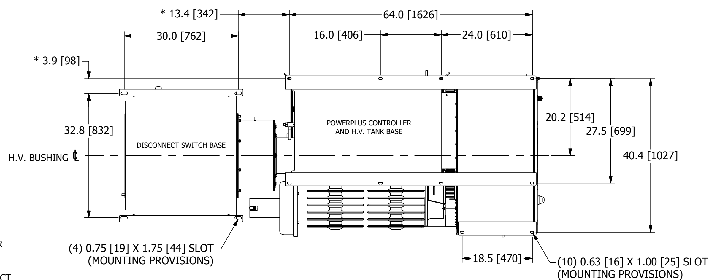
MOUNTING ARRANGEMENT FROM BOTTOM VIEW (SECTION B-B) * FOR REFERENCE ONLY. POWERPLUS AND SWITCH ASSEMBLY MUST BE FIELD FITTED TO THE H. V. DUCT WORK PRIOR TO SECURING TO ROOF.
