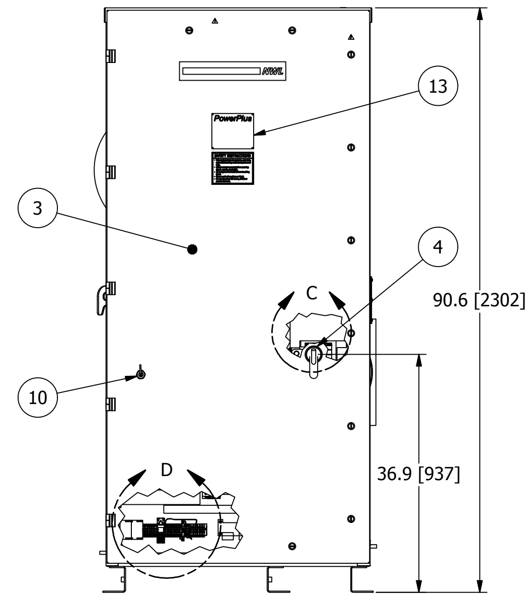
FRONT VIEW
