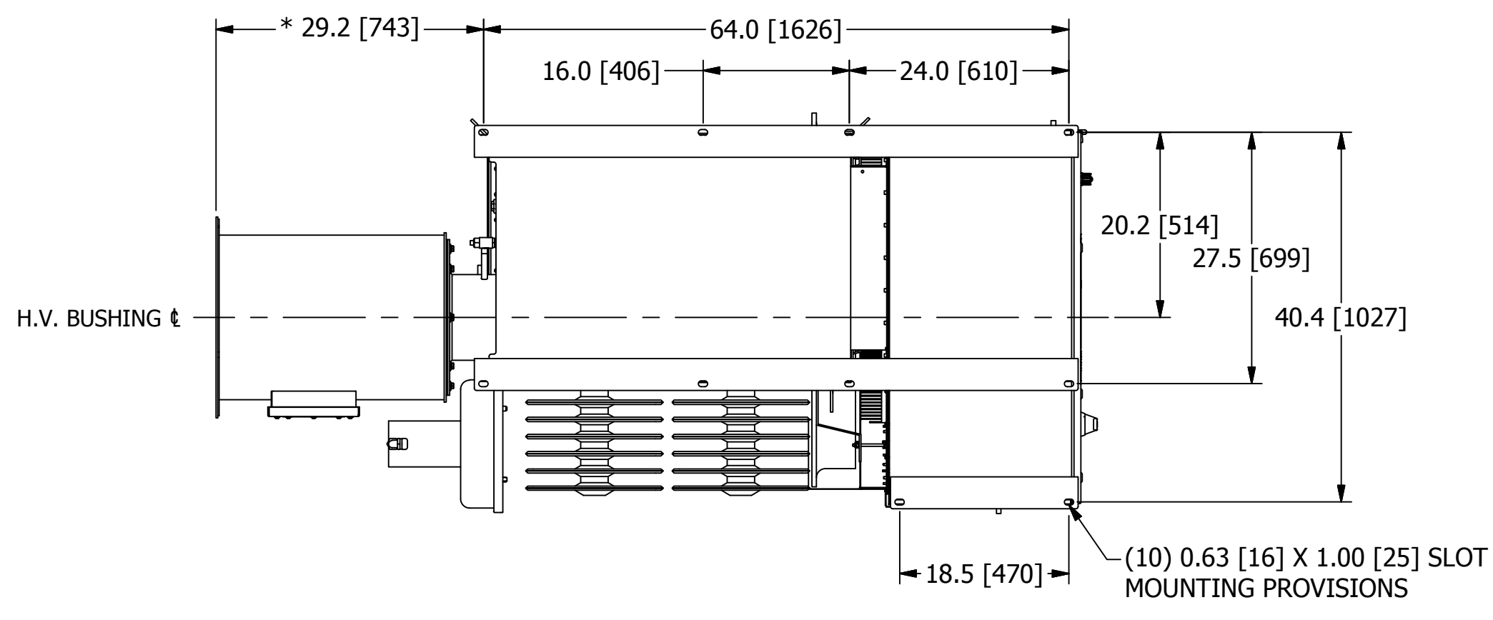
MOUNTING ARRANGEMENT FROM BOTTOM VIEW (SECTION B-B)
