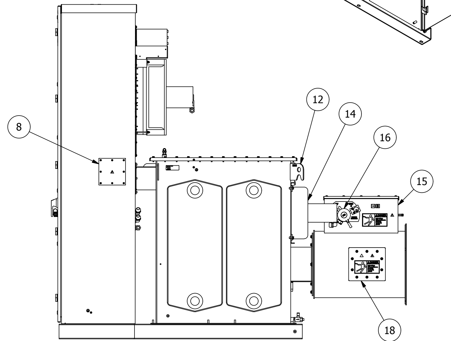
RIGHT VIEW
