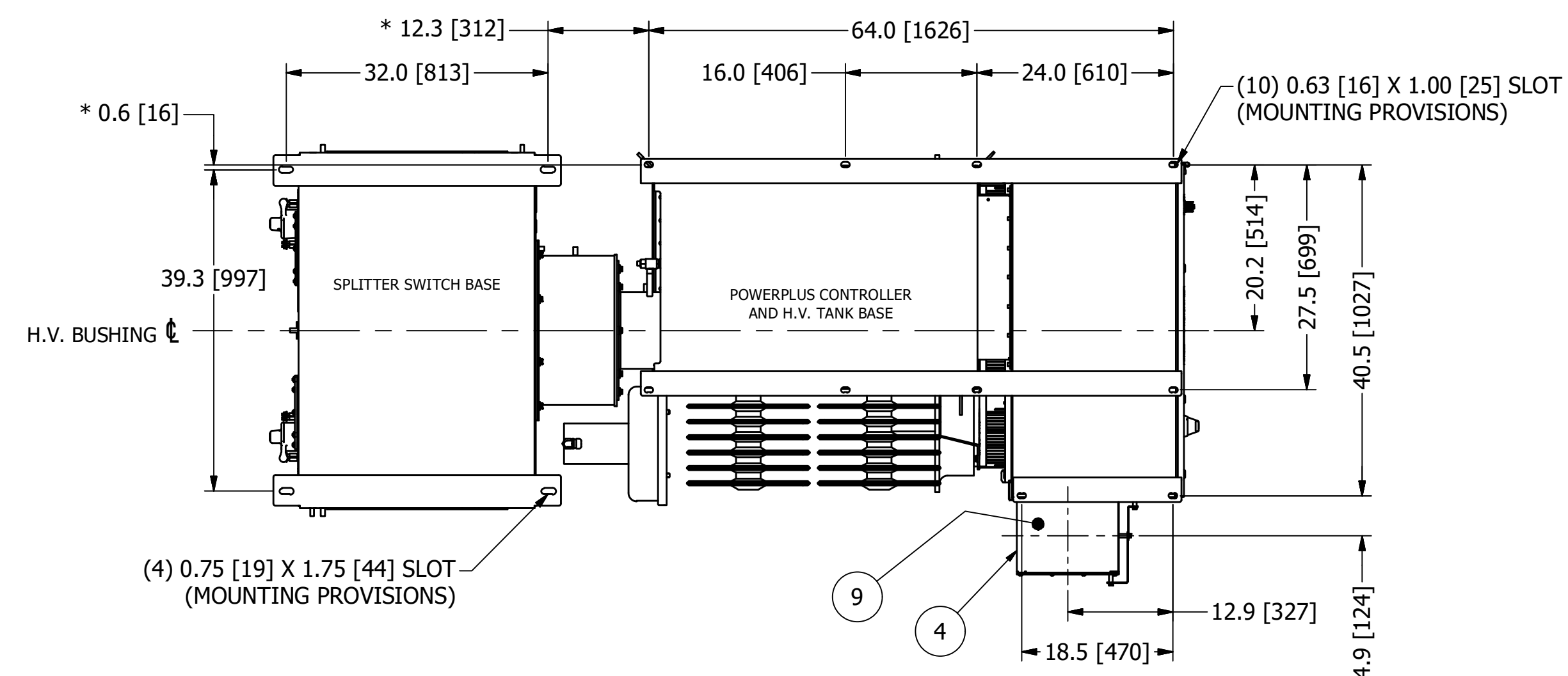
MOUNTING ARRANGEMENT FROM BOTTOM VIEW (SECTION B-B) * FOR REFERENCE ONLY. POWERPLUS AND SWITCH ASSEMBLY MUST BE FIELD FITTED TO THE H. V. DUCT WORK PRIOR TO SECURING TO ROOF.
