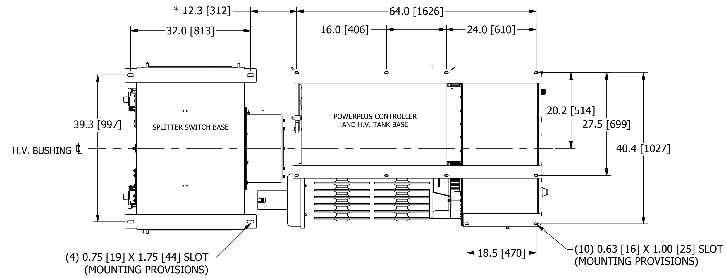
MOUNTING ARRANGEMENT FROM BOTTOM VIEW (SECTION B-B)
