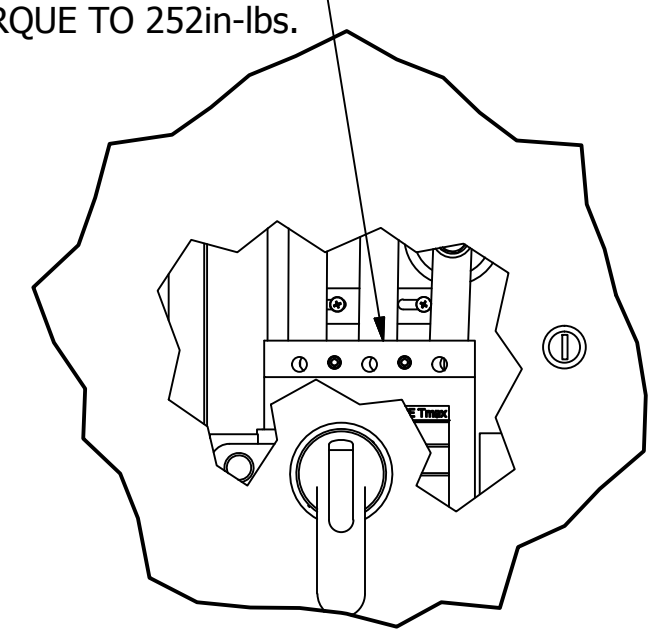
DETAIL C SCALE 1/5 CIRCUIT BREAKER DETAIL
