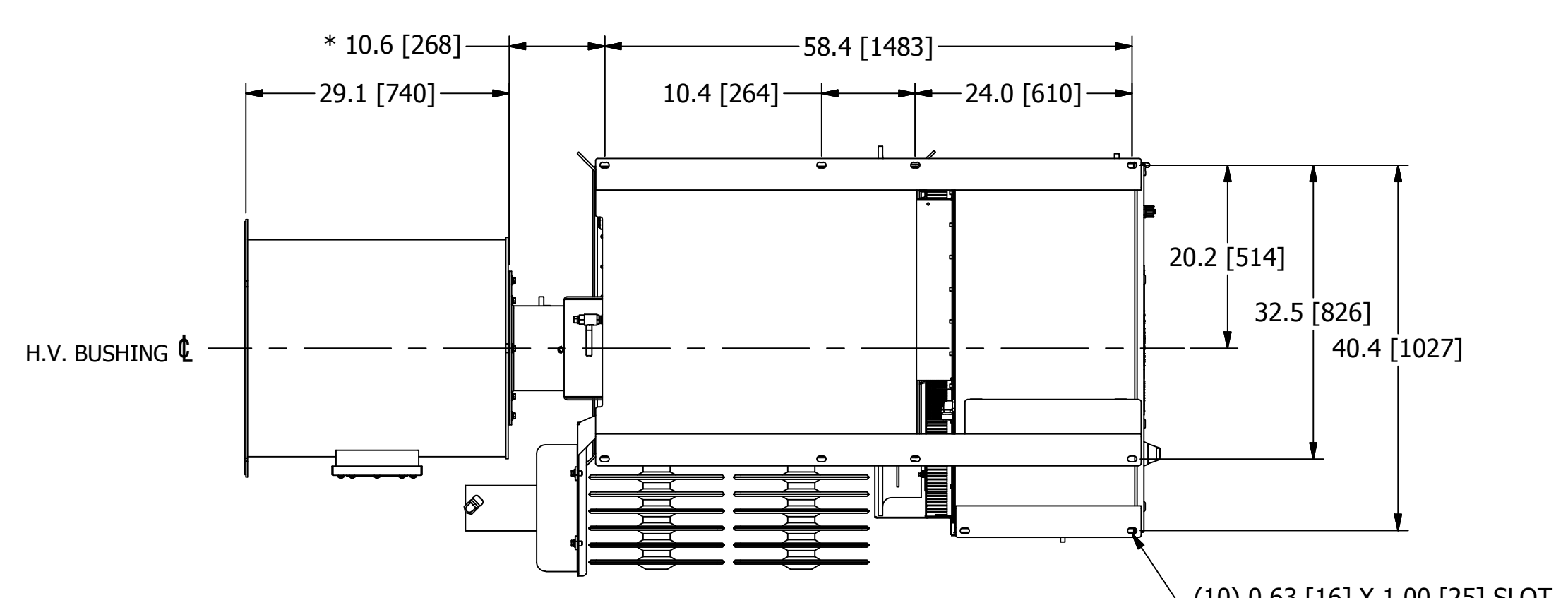
MOUNTING ARRANGEMENT FROM BOTTOM VIEW (VIEW B-B)
