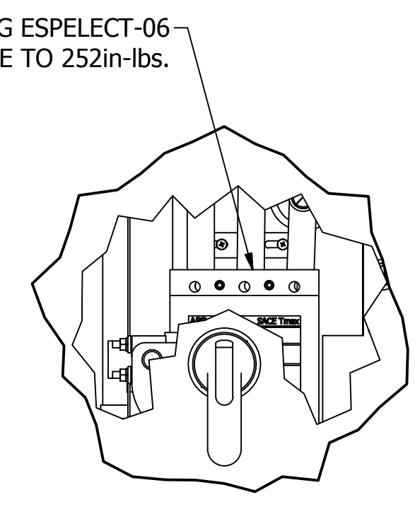
DETAIL C CIRCUIT BREAKER DETAIL SCALE 1 / 5
