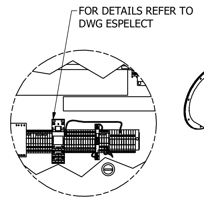
DETAIL D SCALE 1 / 5 2TB' TERMINAL BLOCK RAIL ASSEMBLY
