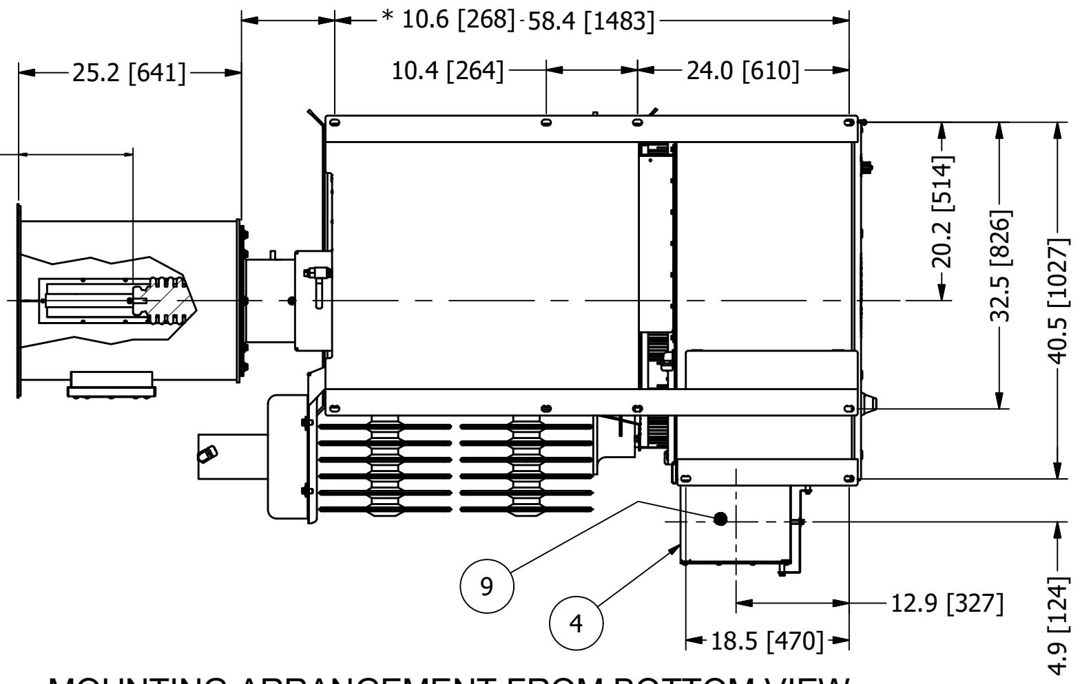
MOUNTING ARRANGEMENT FROM BOTTOM VIEW (VIEW B-B)
