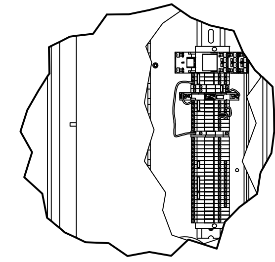
DETAIL D '2TB' TERMINAL BLOCK RAIL ASSY SCALE 1/5
