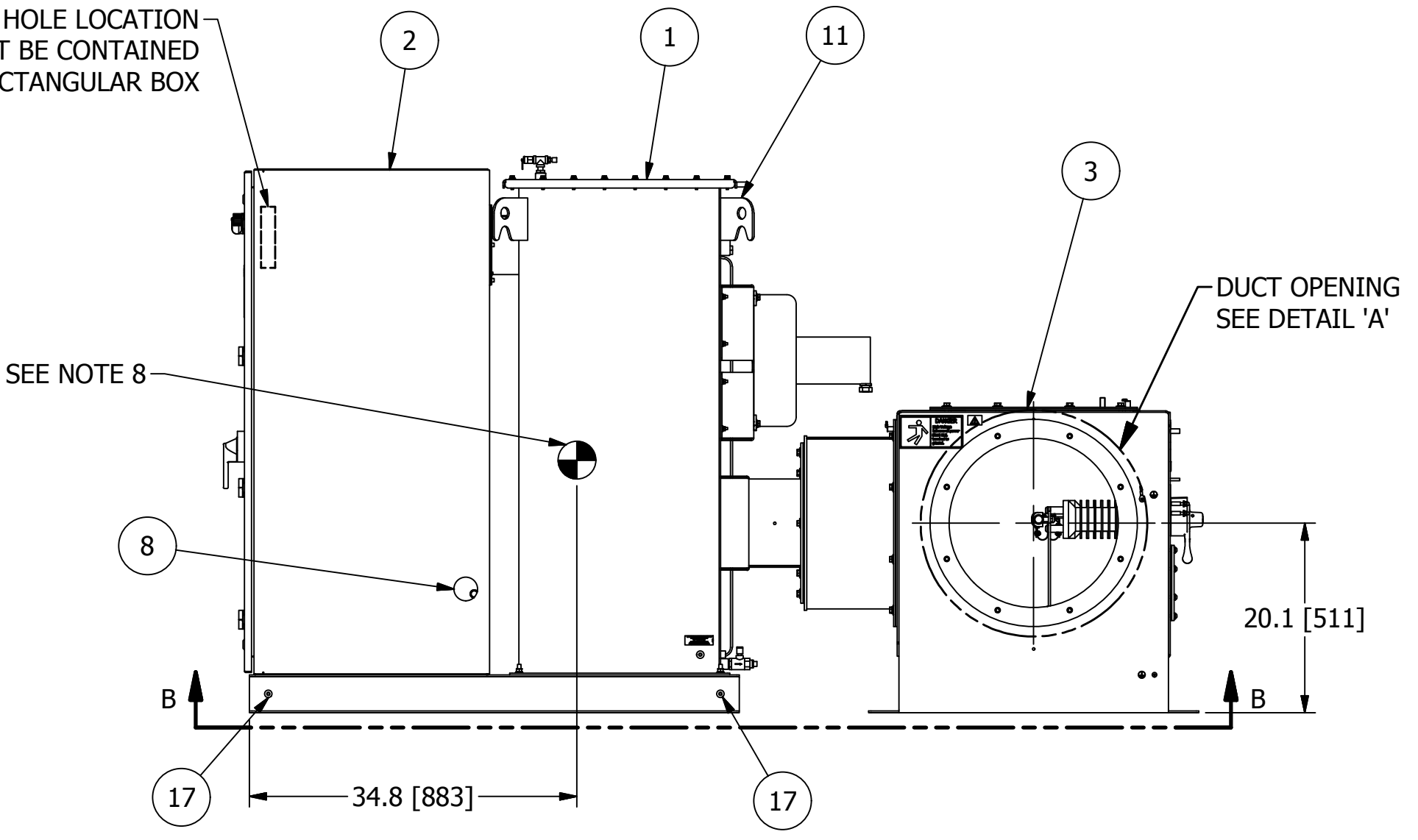
RIGHT VIEW
