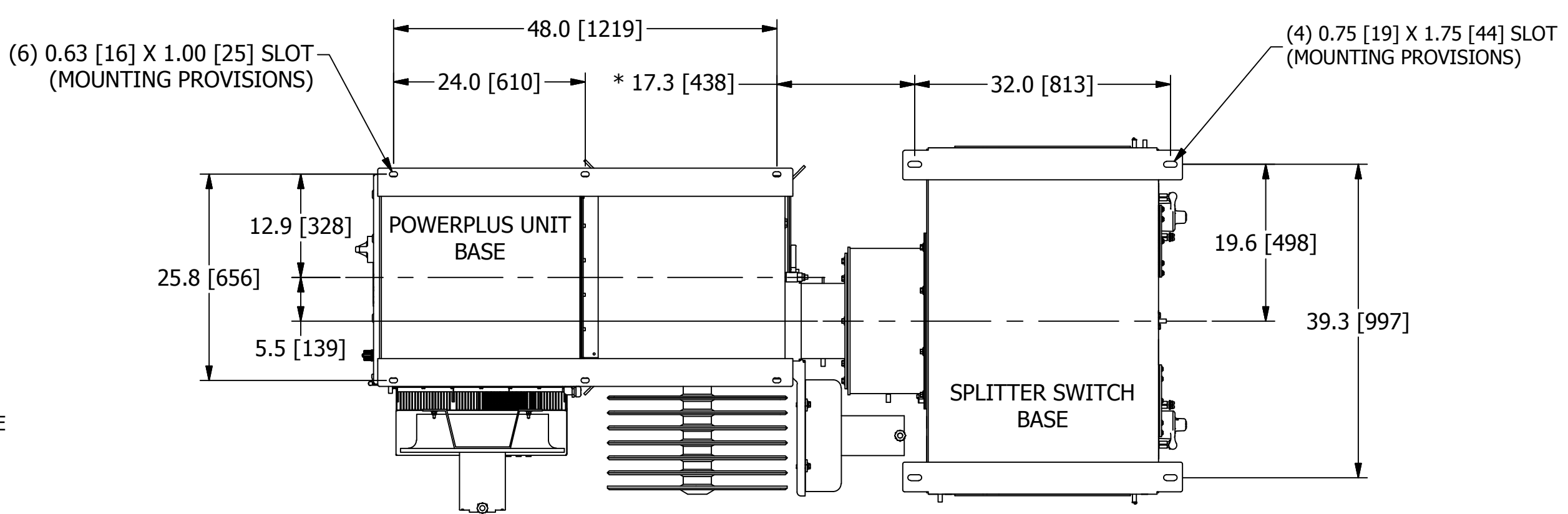
MOUNTING ARRANGEMENT FROM BOTTOM VIEW (SECTION B-B)
