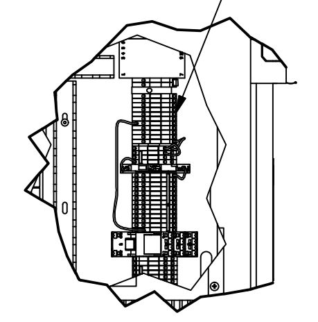
DETAIL D TERMINAL BLOCK RAIL ASSEMBLY SCALE 1 / 6
