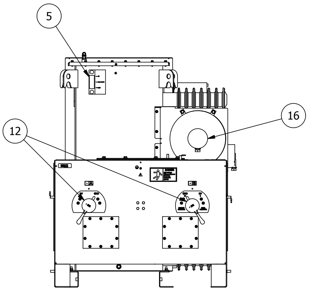
REAR VIEW
