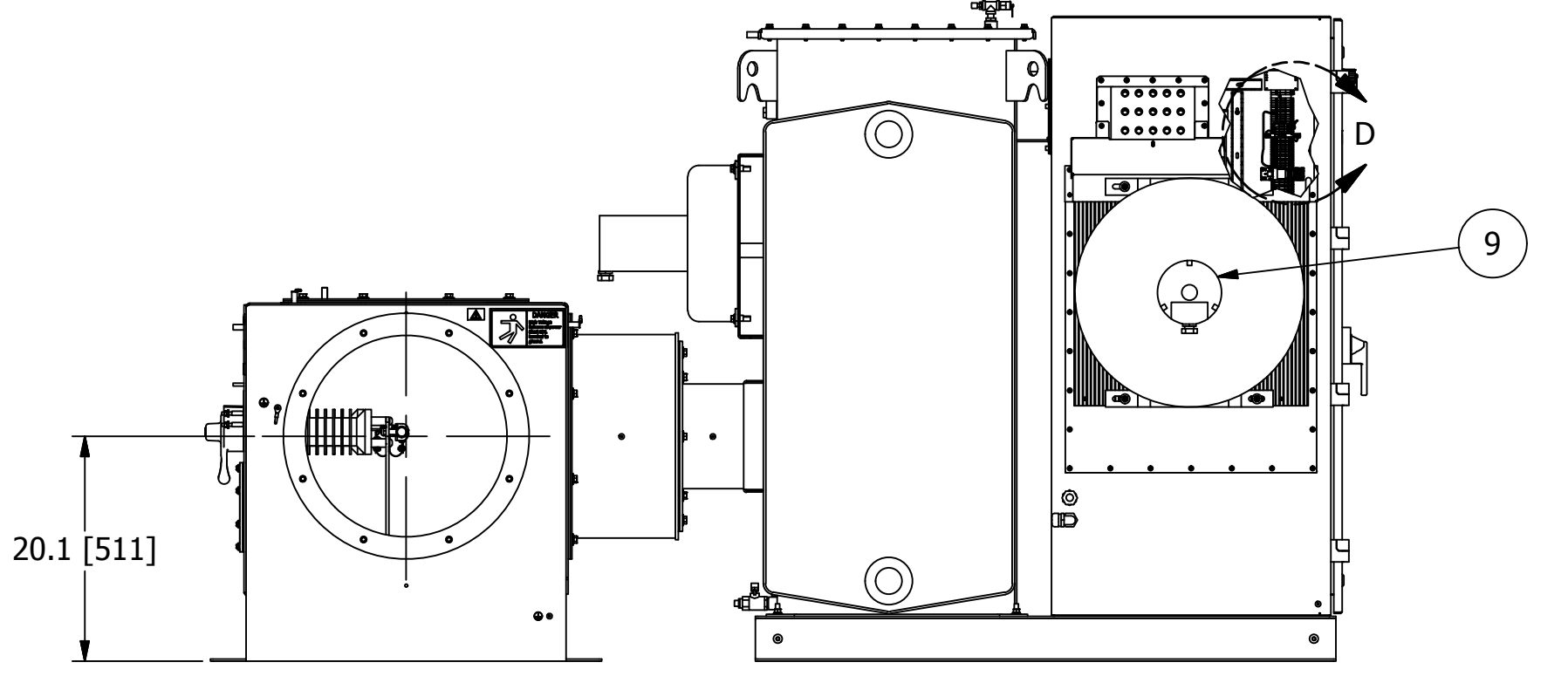
LEFT VIEW
